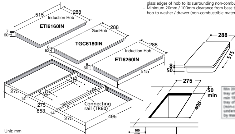
Installation drawing for 3 sets of domino hobs
